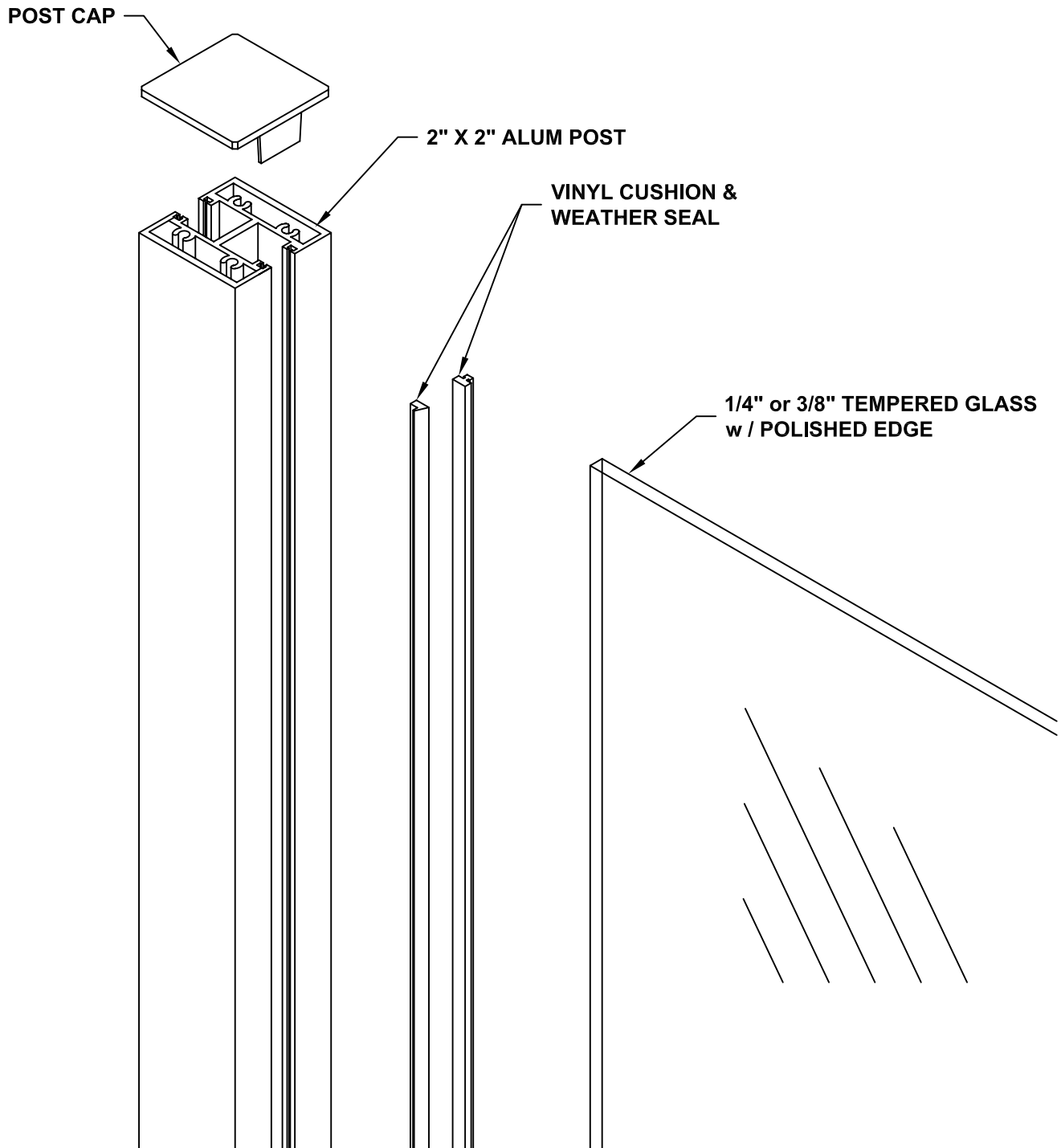
GLASS POOL ENCLOSURE - DETAIL 1
