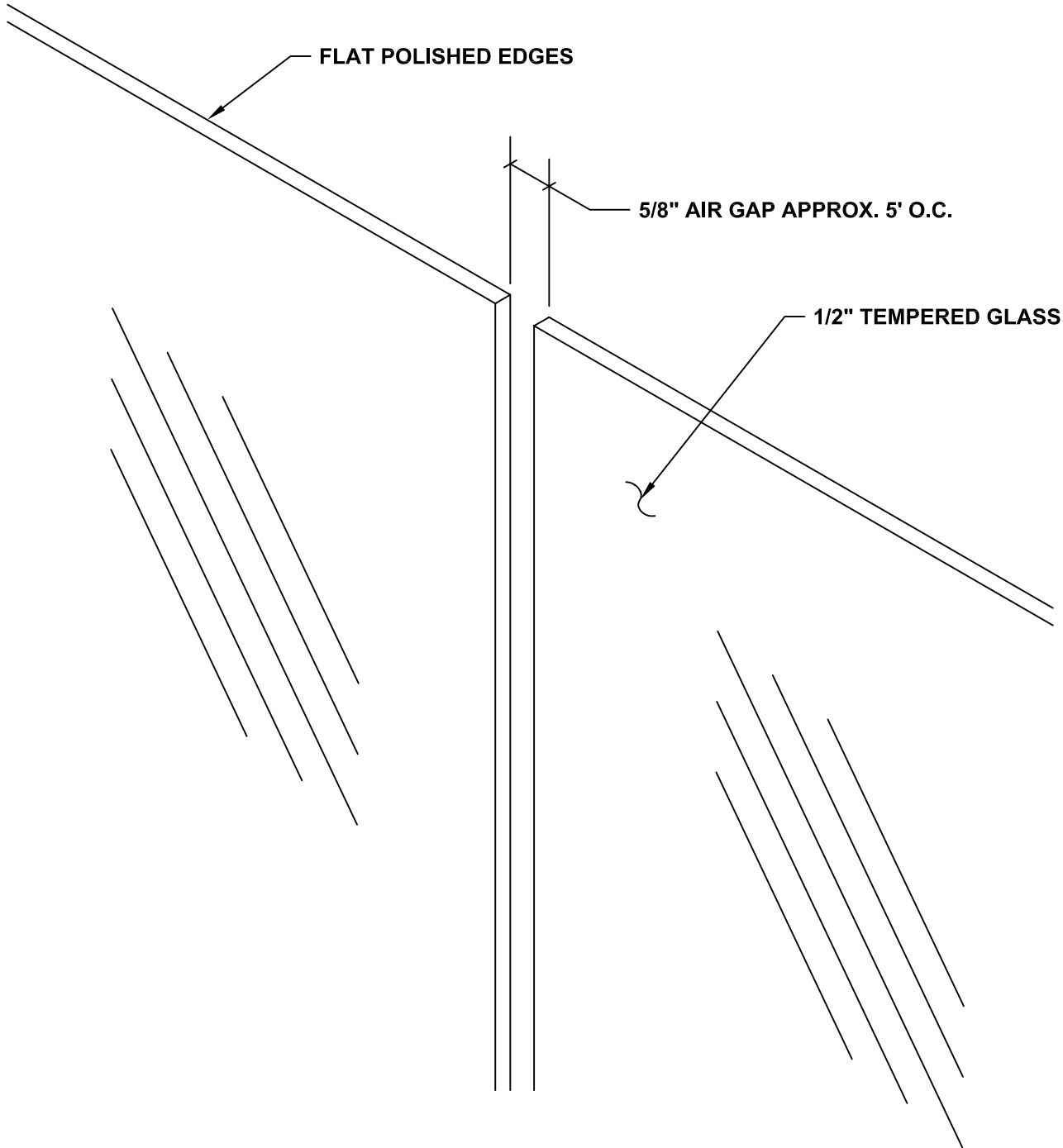
FRAMELESS GLASSWALL - DETAIL 1
