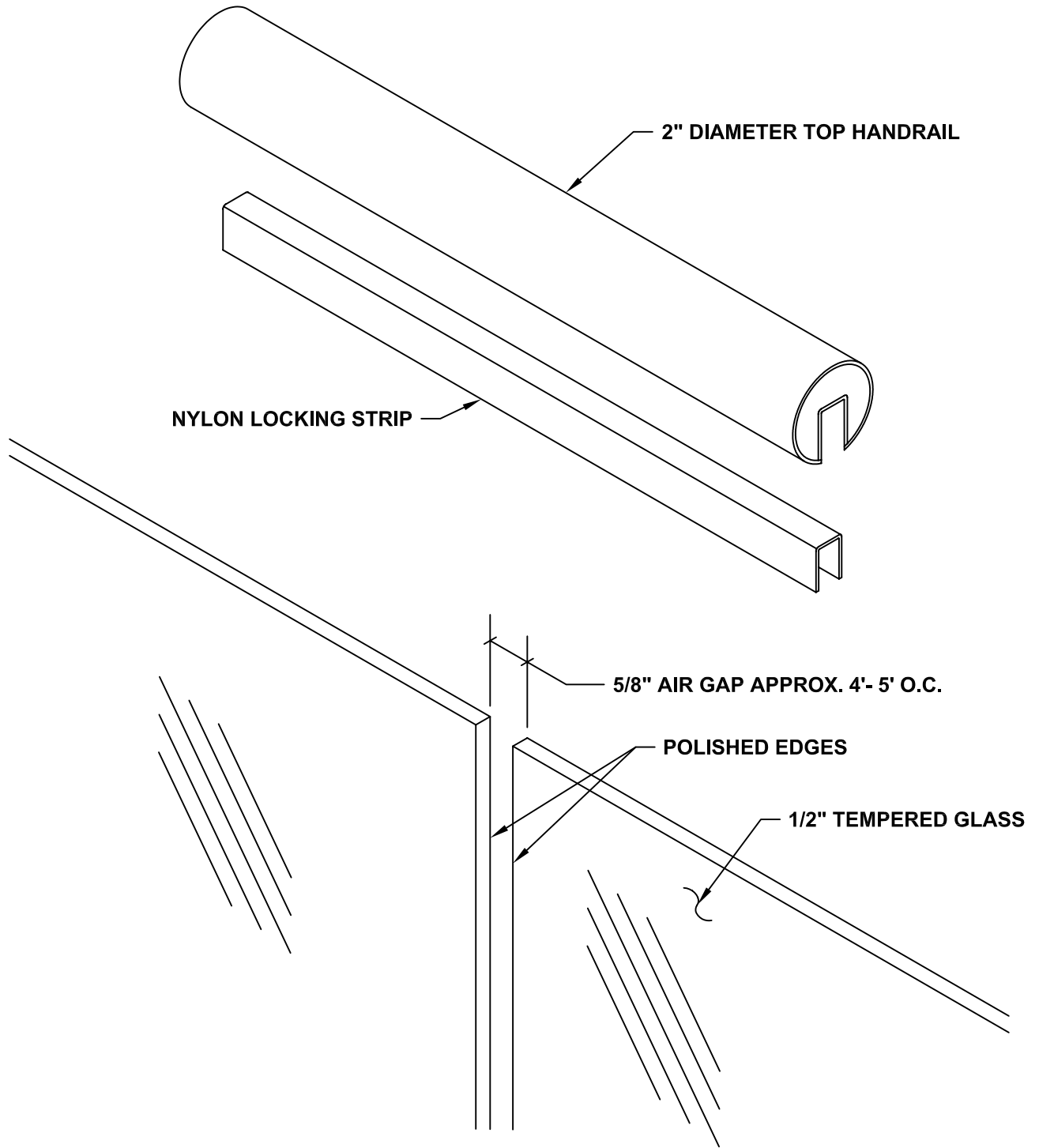
FRAMELESS GLASS HANDRAIL - DETAIL 1
