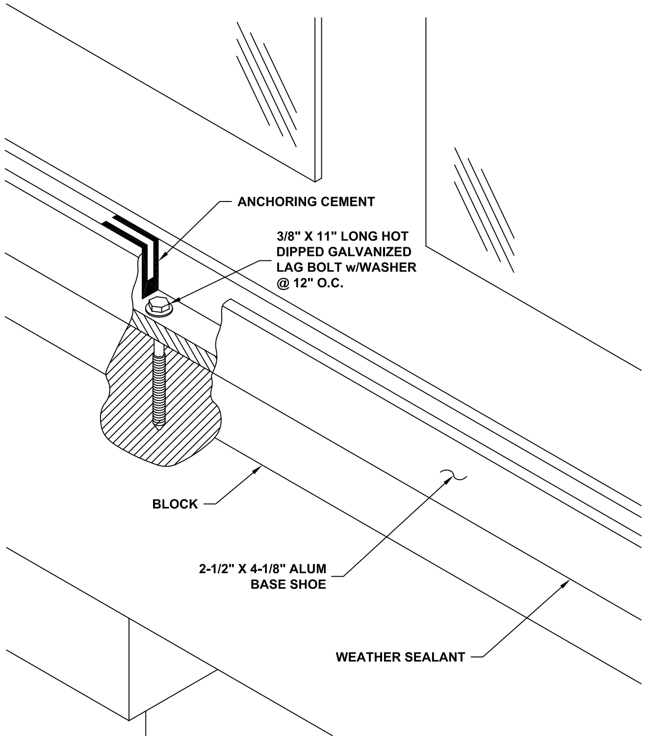
FRAMELESS GLASS HANDRAIL - DETAIL 2
