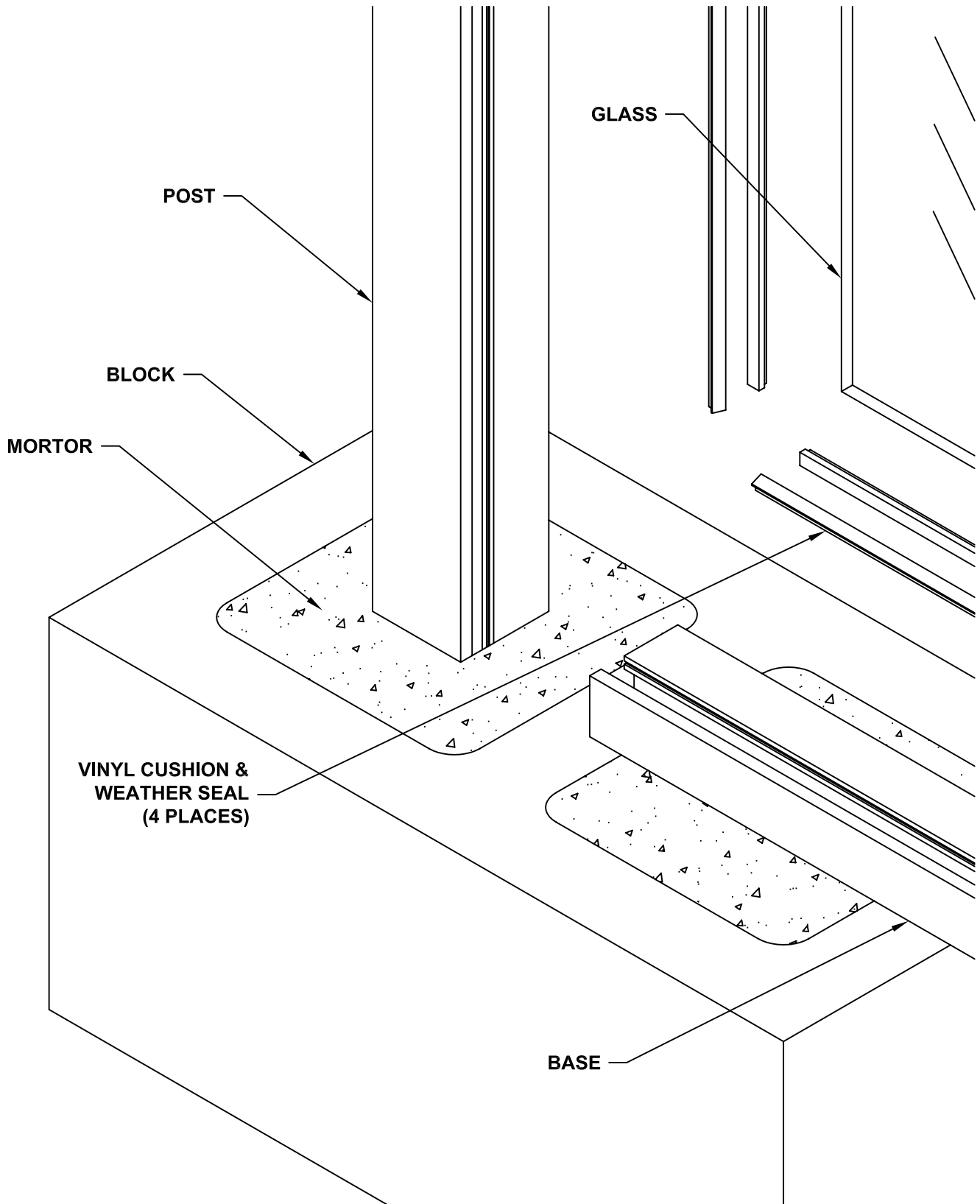
GLASSWALL SERIES - DETAIL 2
