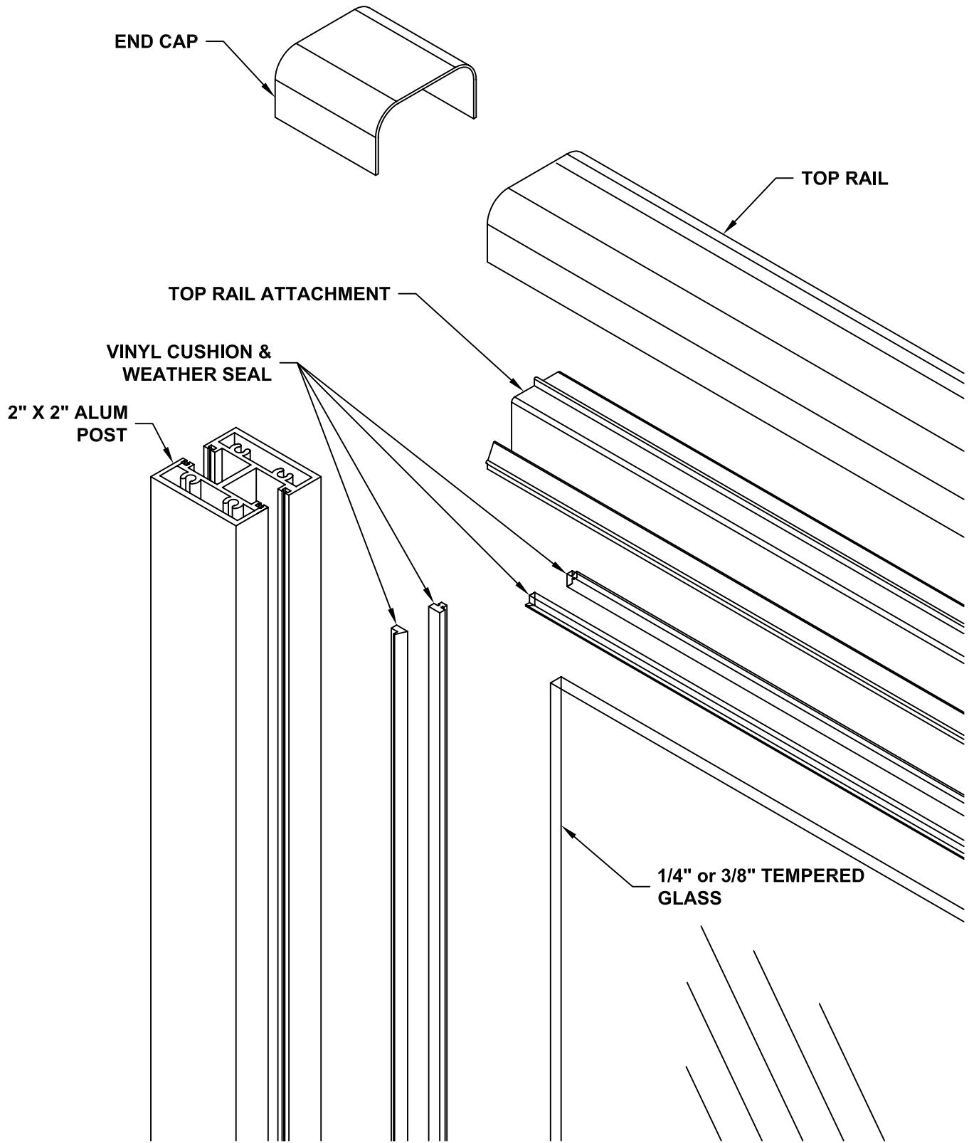
GLASS HANDRAIL SERIES - DETAIL 1
