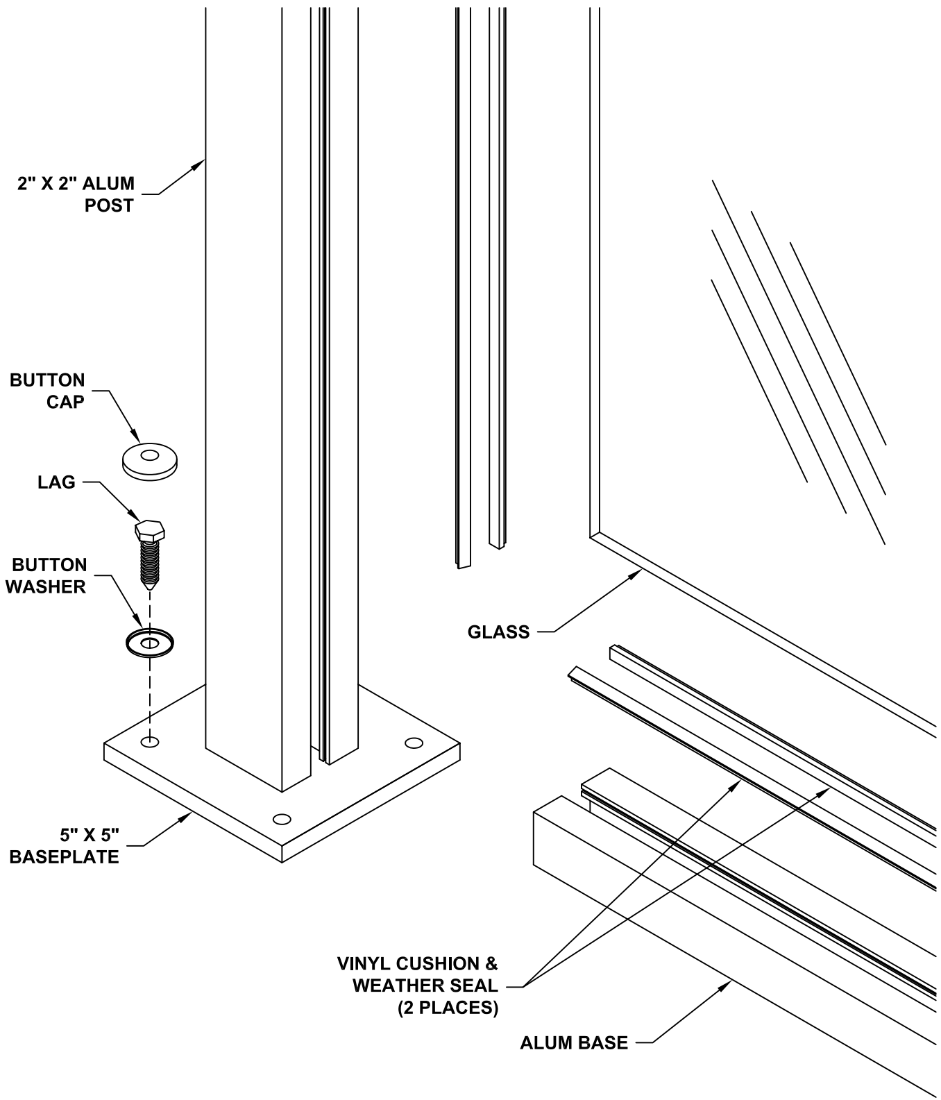
GLASS HANDRAIL SERIES - DETAIL 2
