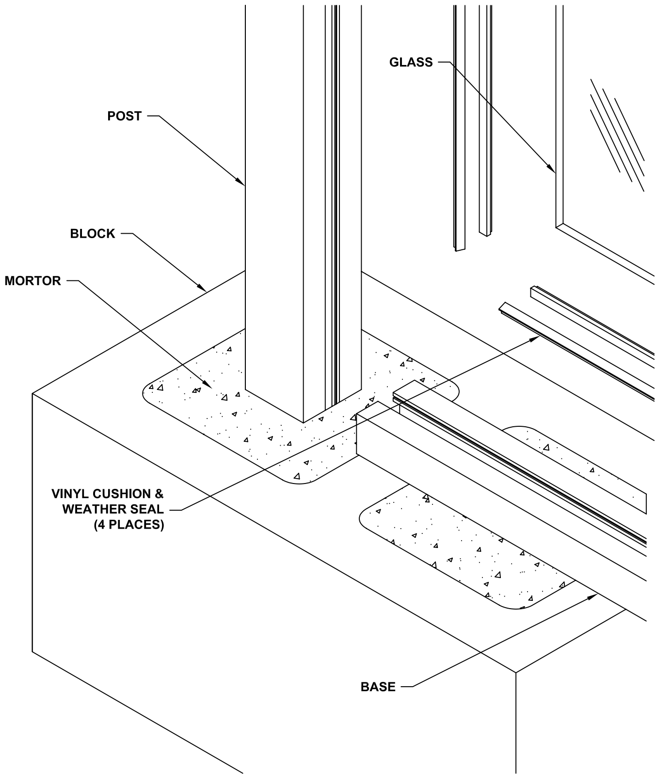
HEAVY GLASS SOUND WALL - DETAIL 2
